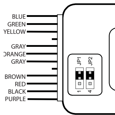
WET OUTPUT ON RELAY 1
