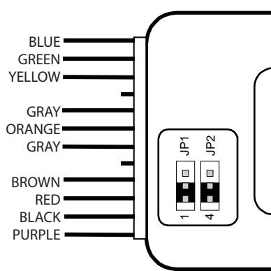
DRY OUTPUT ON RELAY 1
